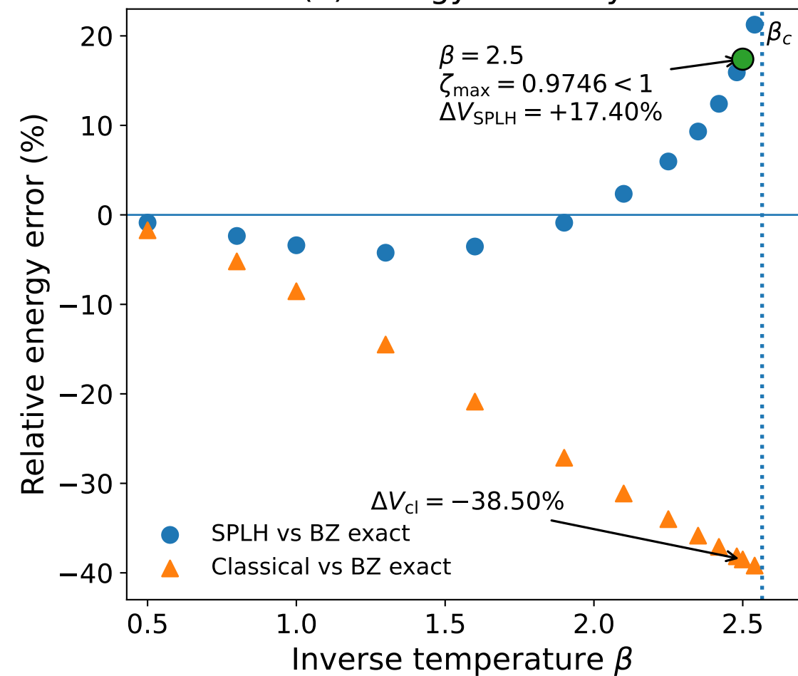
(a) Energy accuracy
