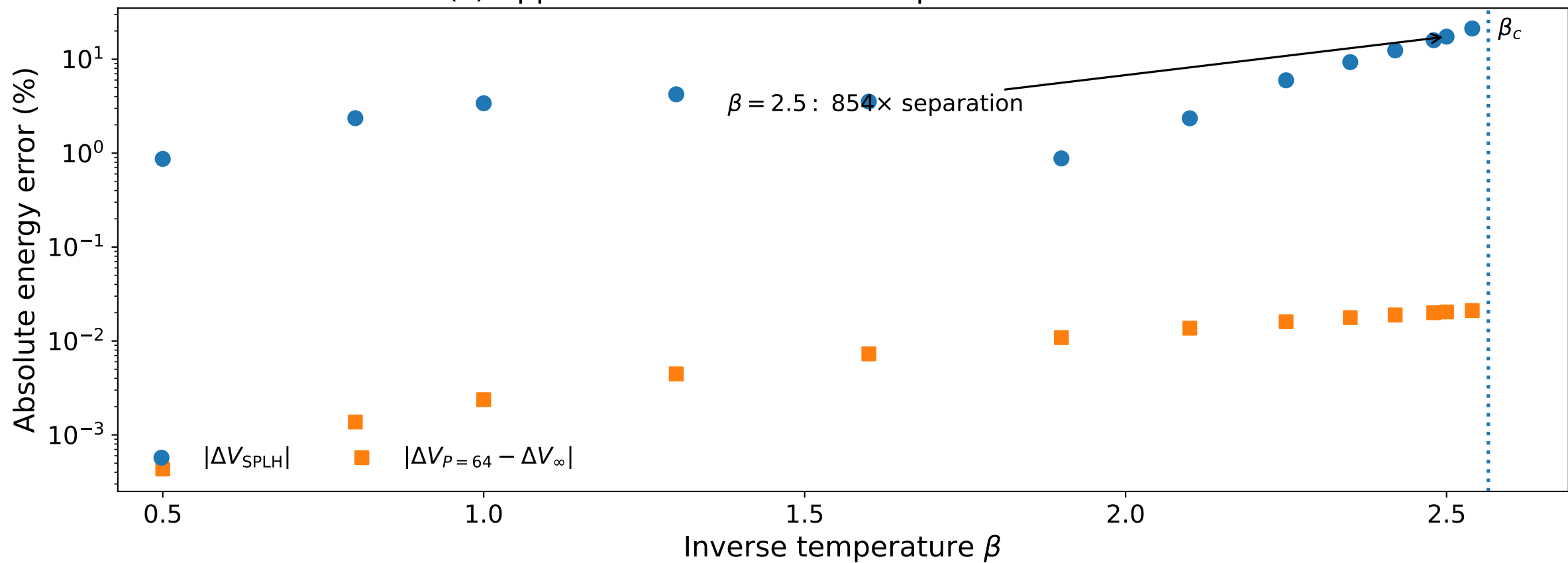
(c) Approximation error versus primitive Trotter error
