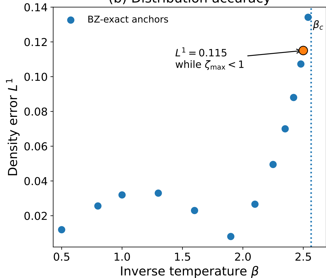
(b) Distribution accuracy
