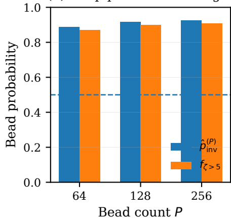
(b) Deep post-caustic weight
