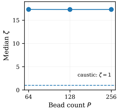
(c) Instability depth
