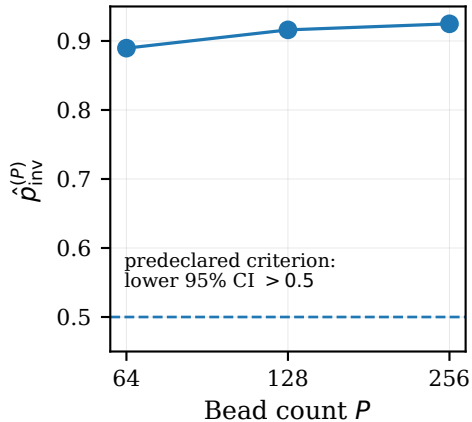
(a) Invalid occupation
