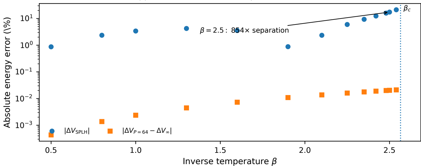
(c) Approximation error versus primitive Trotter error
