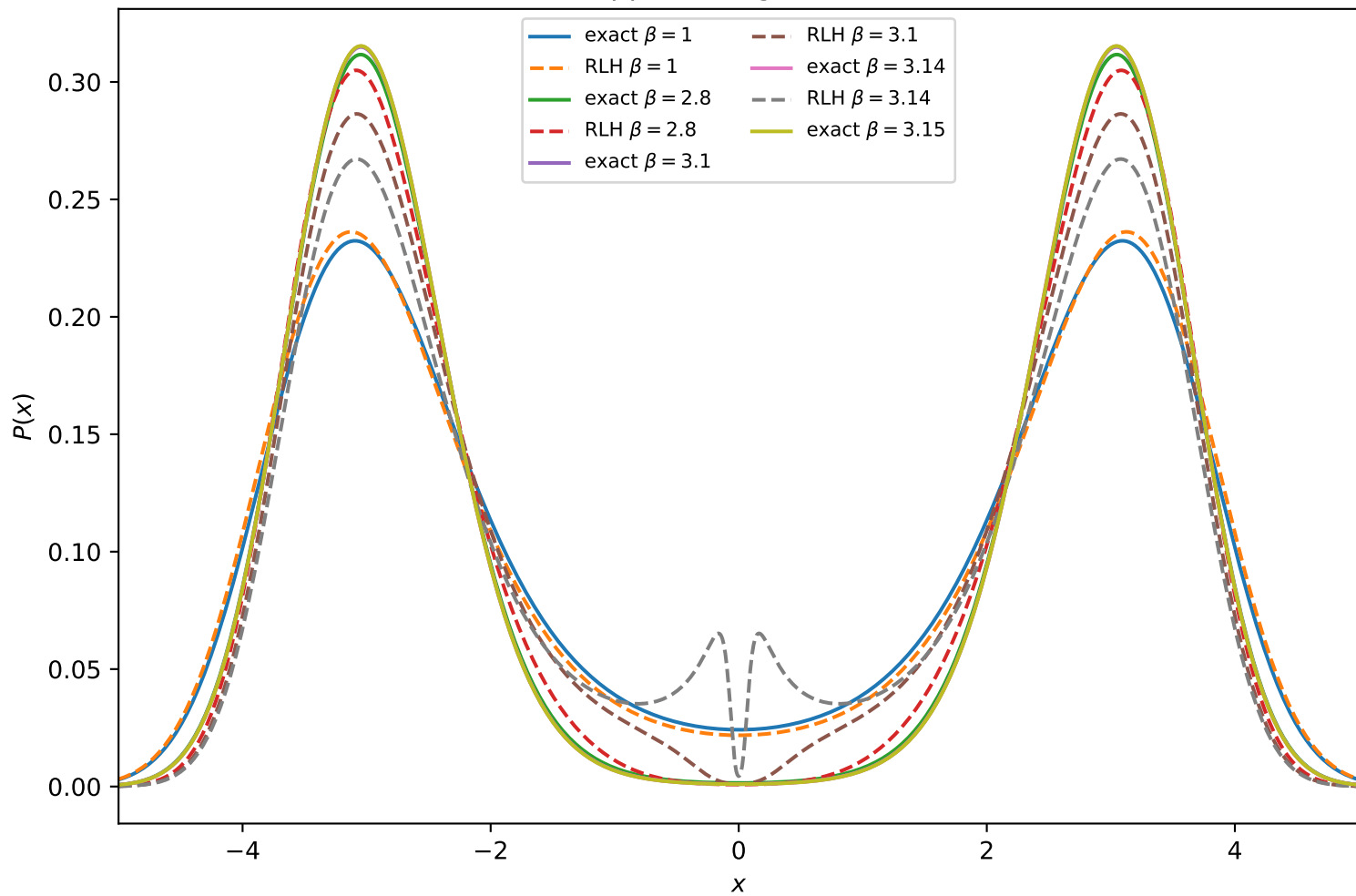
Global double well approaching the local Gaussian caustic
