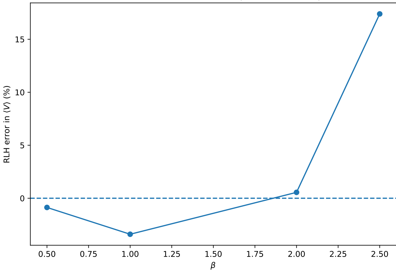
Observable-level error on the periodic landscape
