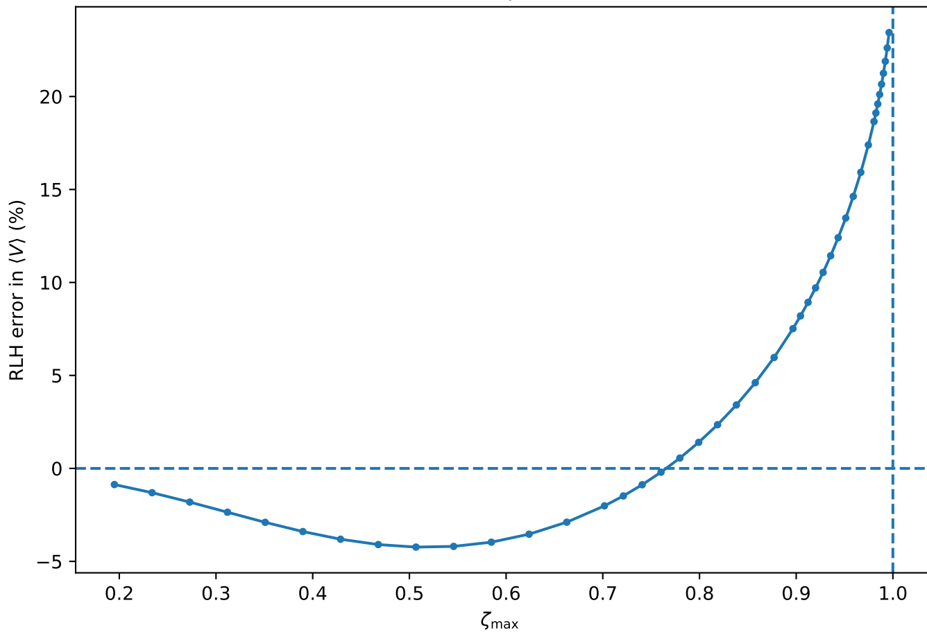
Observable-level pre-caustic error
