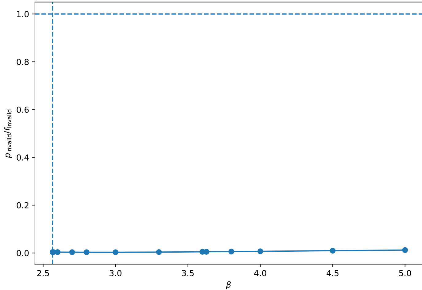
Quantum occupation of the Gaussian-invalid region
