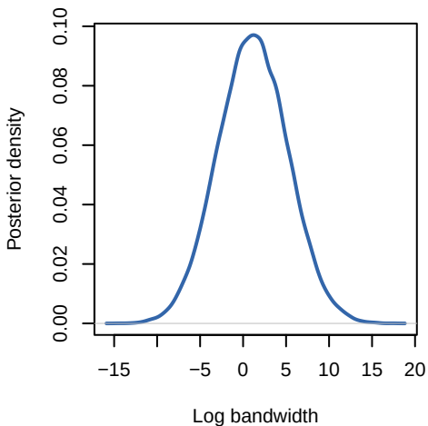
continuous_1 bandwidth posterior
