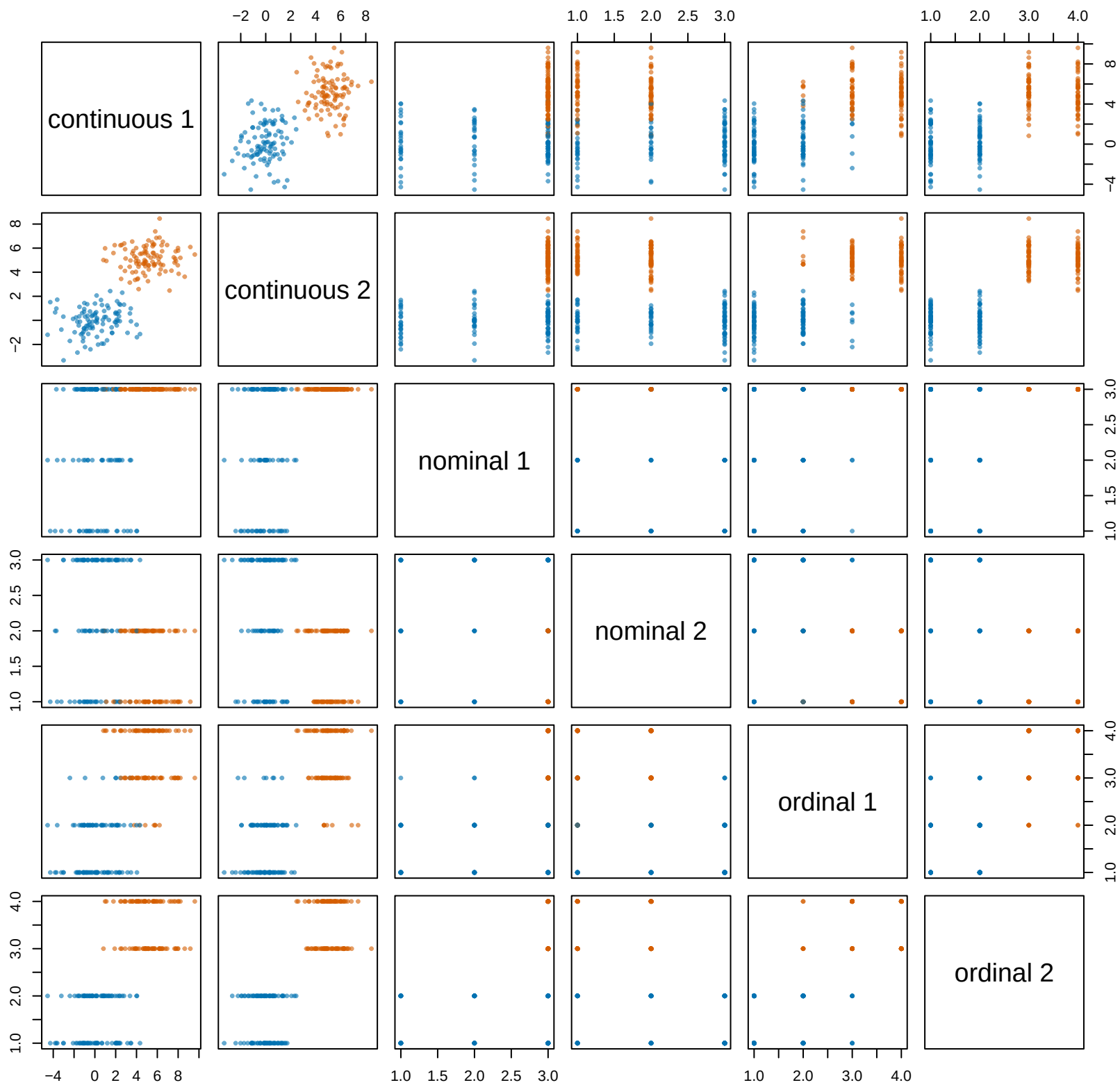
Simulated mixed-type data Cluster 1 (blue), Cluster 2 (orange)
