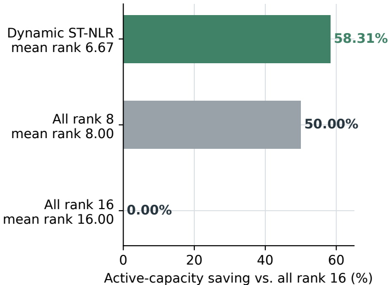
(a) Feasible capacity under 2% tolerance
