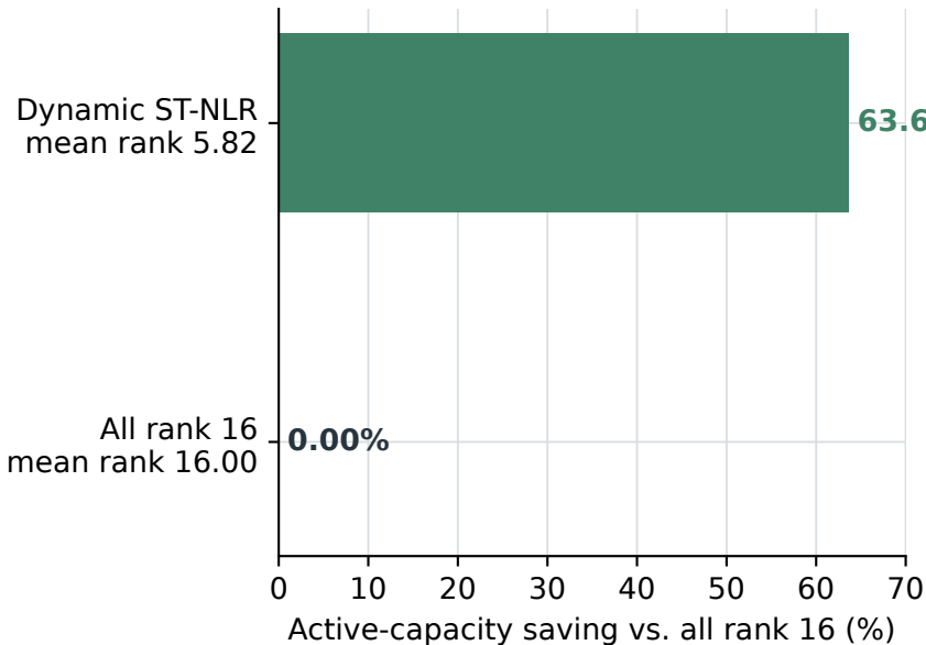
(a) Validation-feasible capacity
