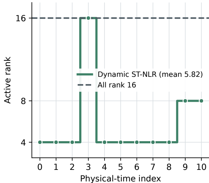
(b) Frozen validation-selected schedule
