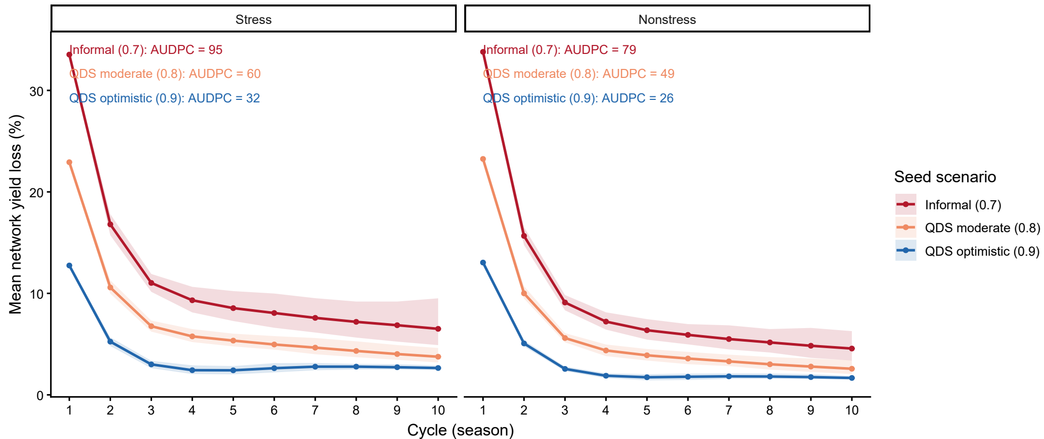
Figure 3. Epidemic trajectories by seed scenario (mean, 5-95% band)
