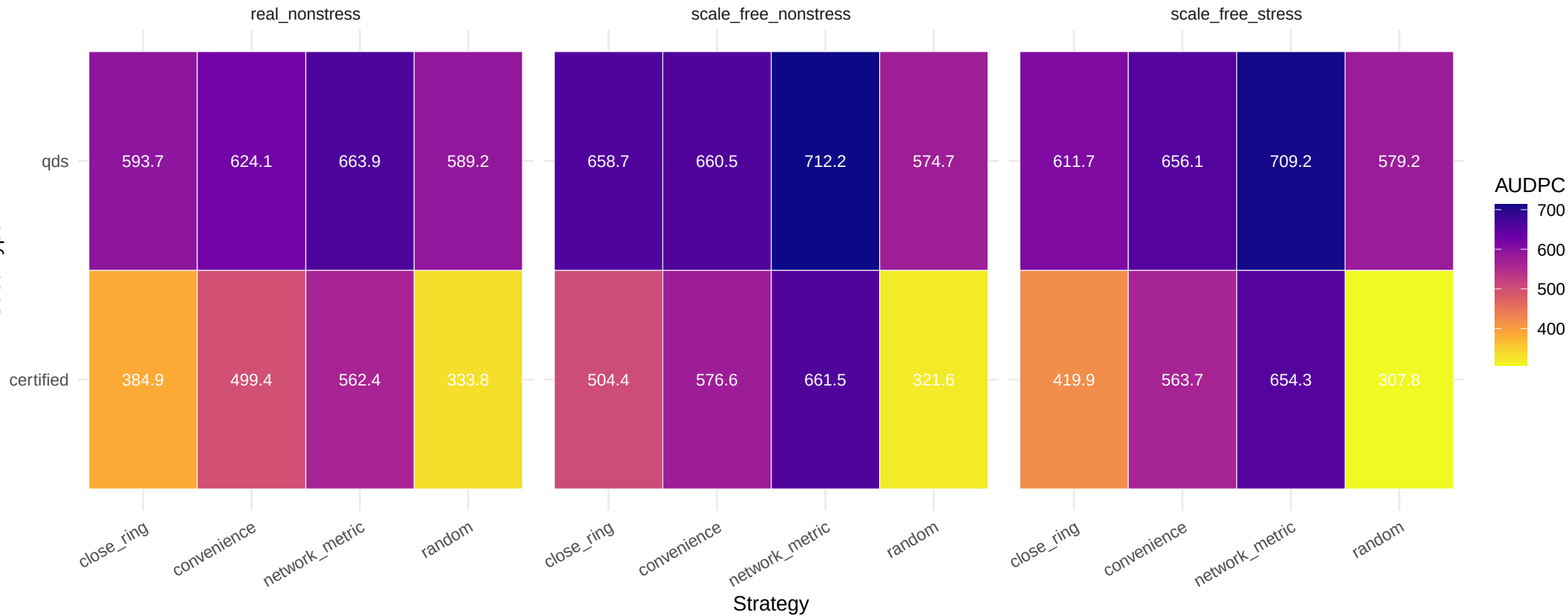
Objective 3: AUDPC by network, seed type, and strategy
