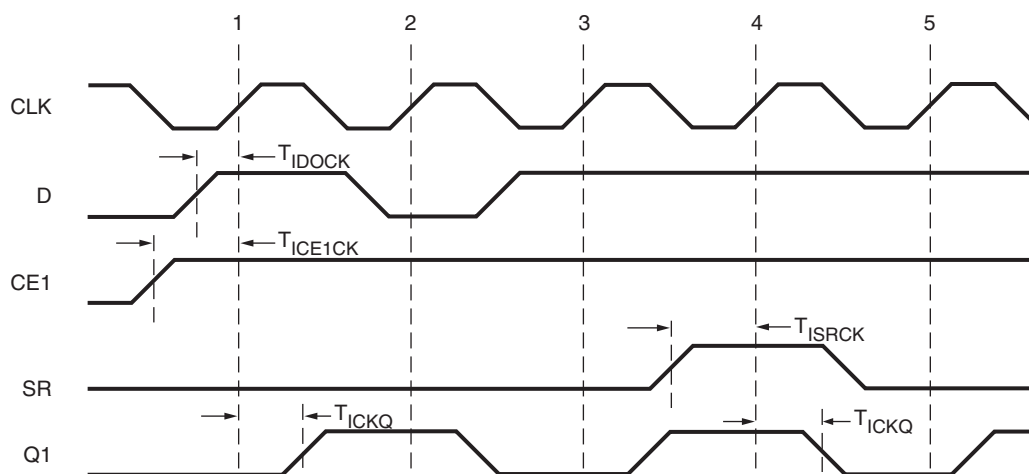
Figure 2-9: ILOGIC Input Register Timing Characteristics
