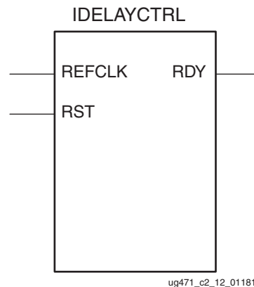
Figure 2-14: IDELAYCTRL Primitive
