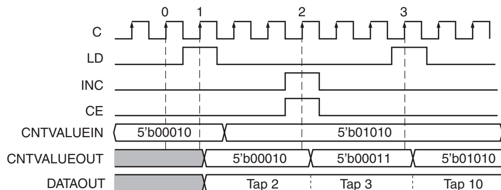
Figure 2-13: IDELAY in VAR_LOAD Timing Diagram
