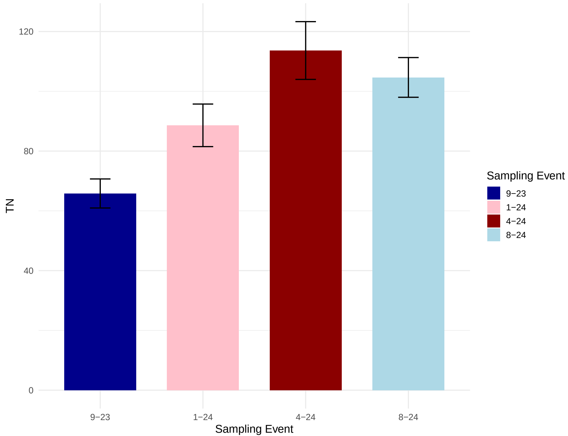
Average TN across Sampling Events
