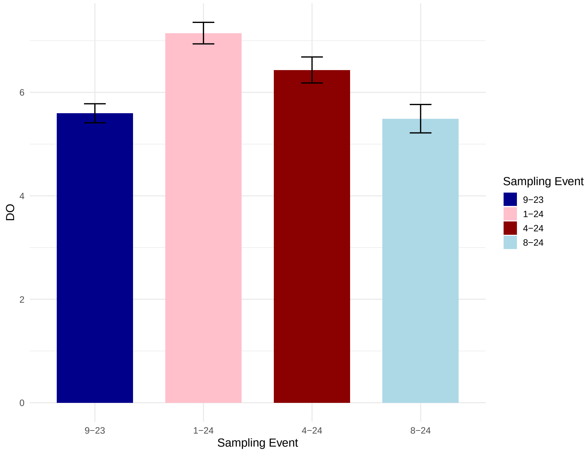
Average DO across Sampling Events
