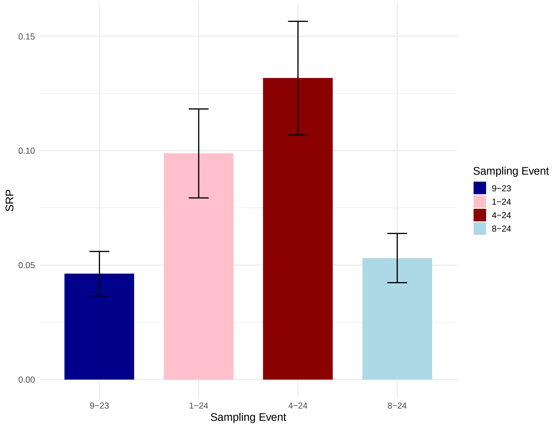
Average SRP across Sampling Events
