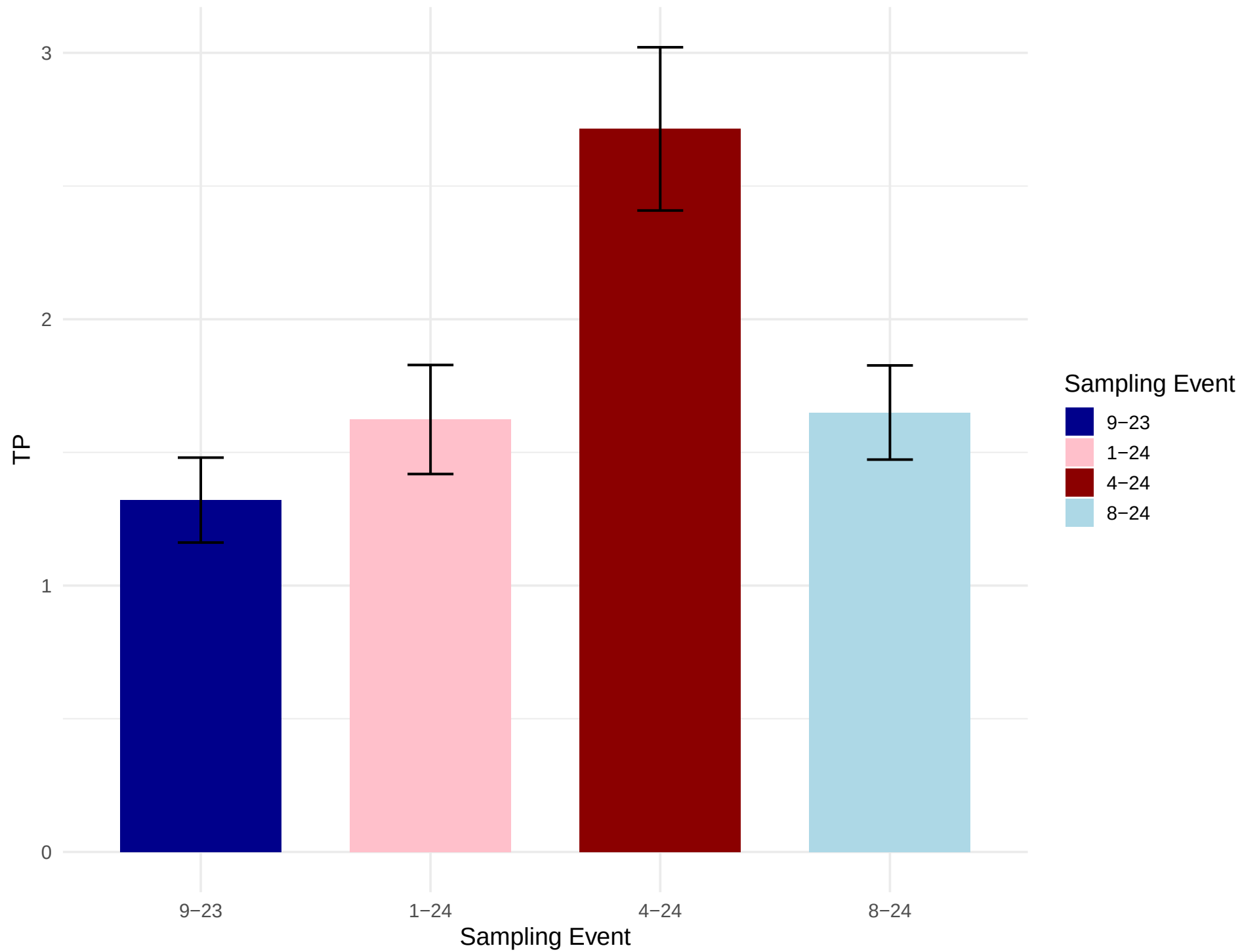
Average TP across Sampling Events
