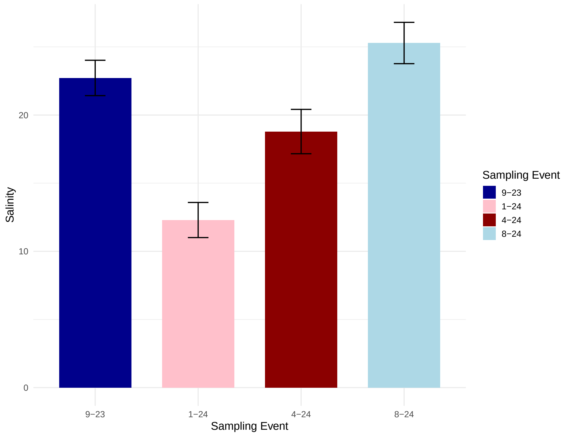
Average Salinity across Sampling Events
