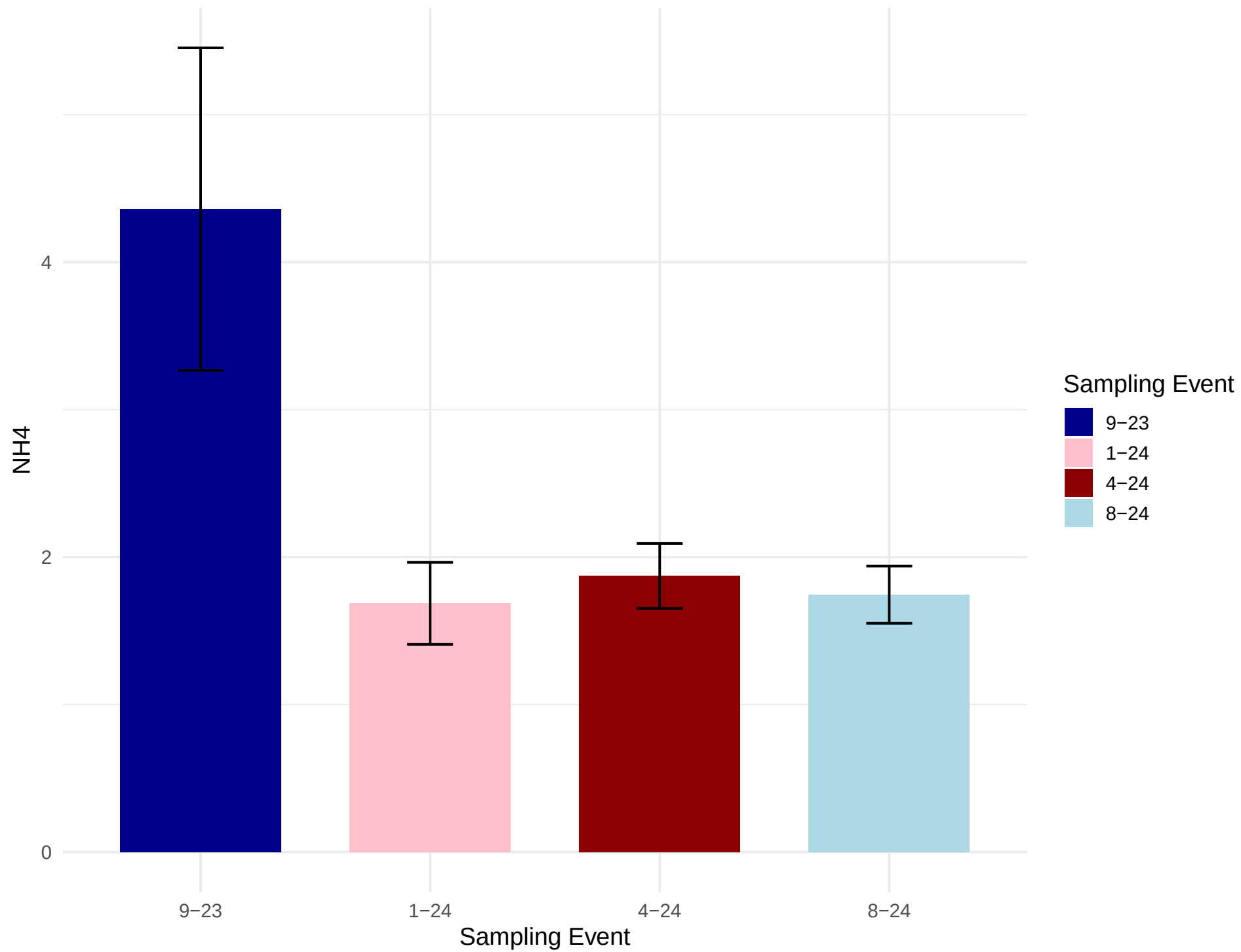
Average NH 4 across Sampling Events
