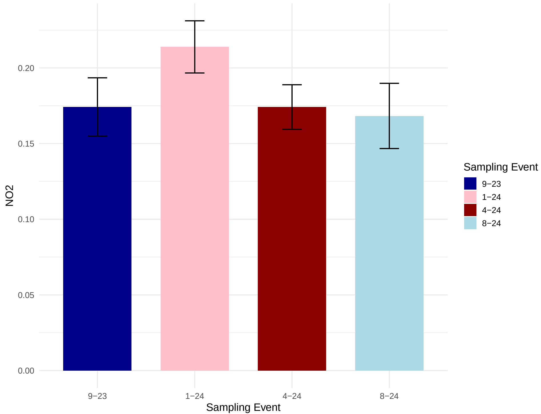
Average NO2 across Sampling Events
