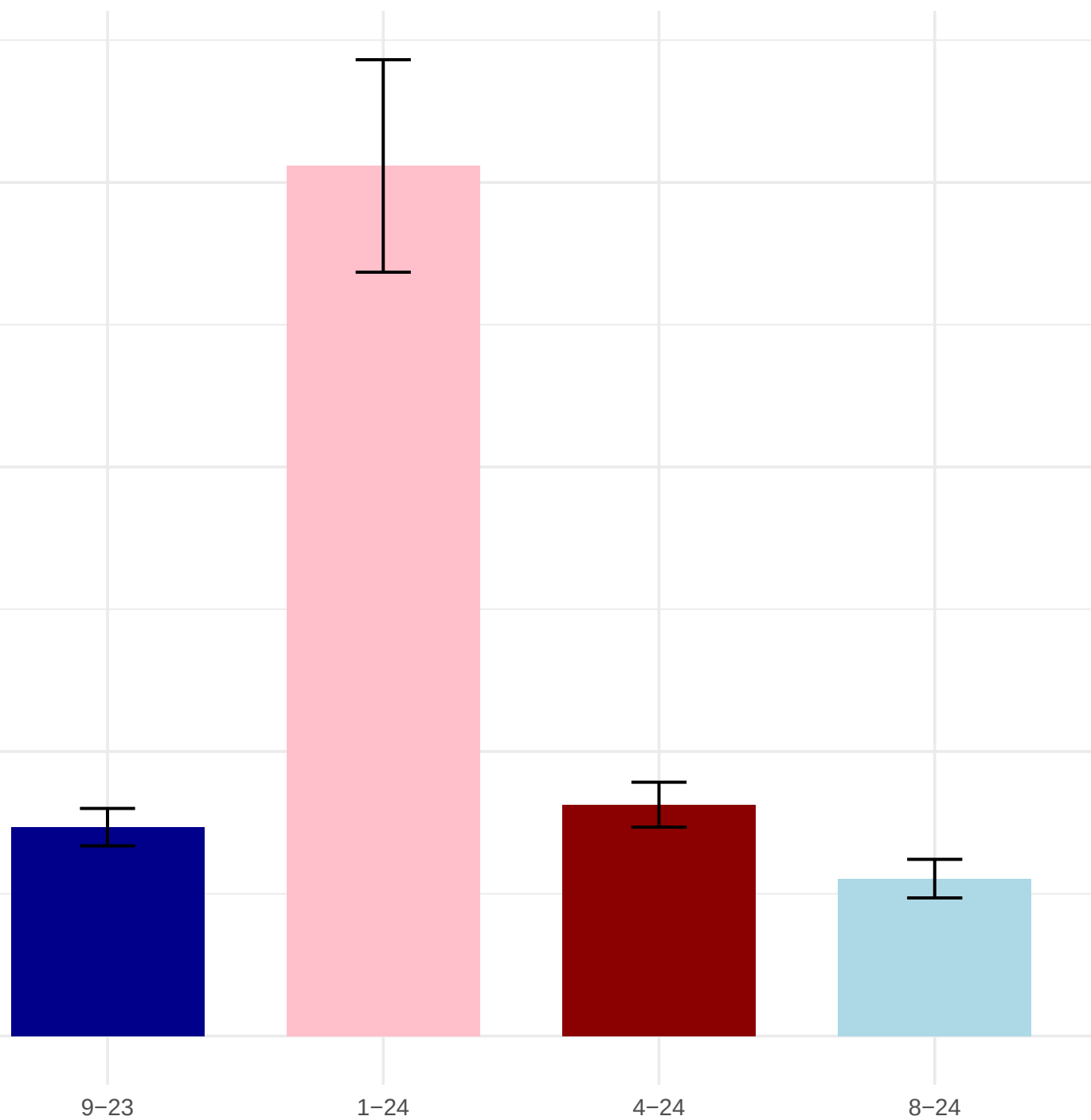
Average Chlorophyll across Sampling Events
