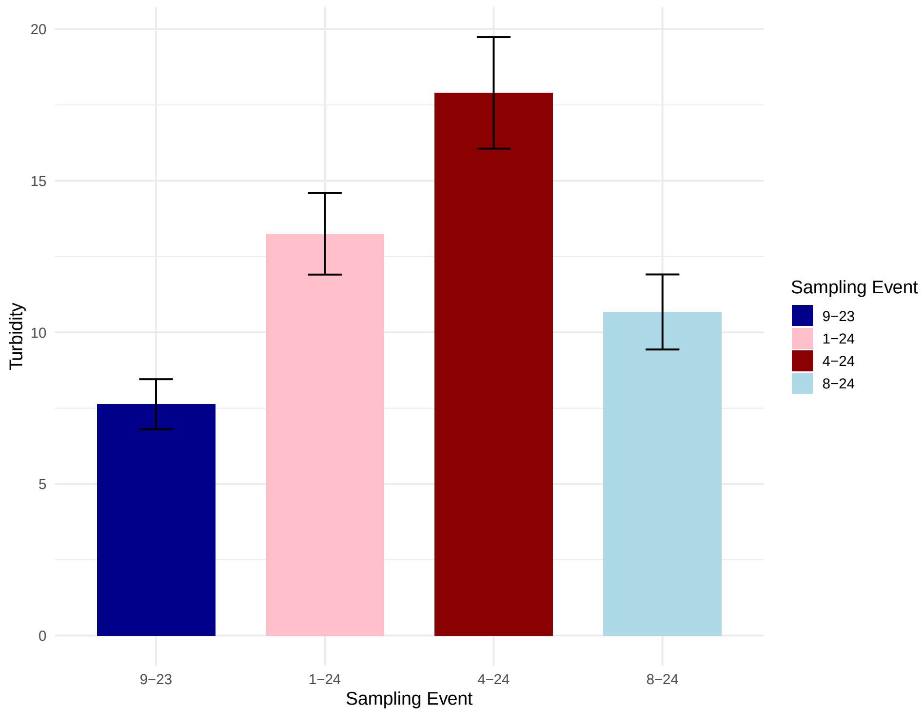
Average Turbidity across Sampling Events
