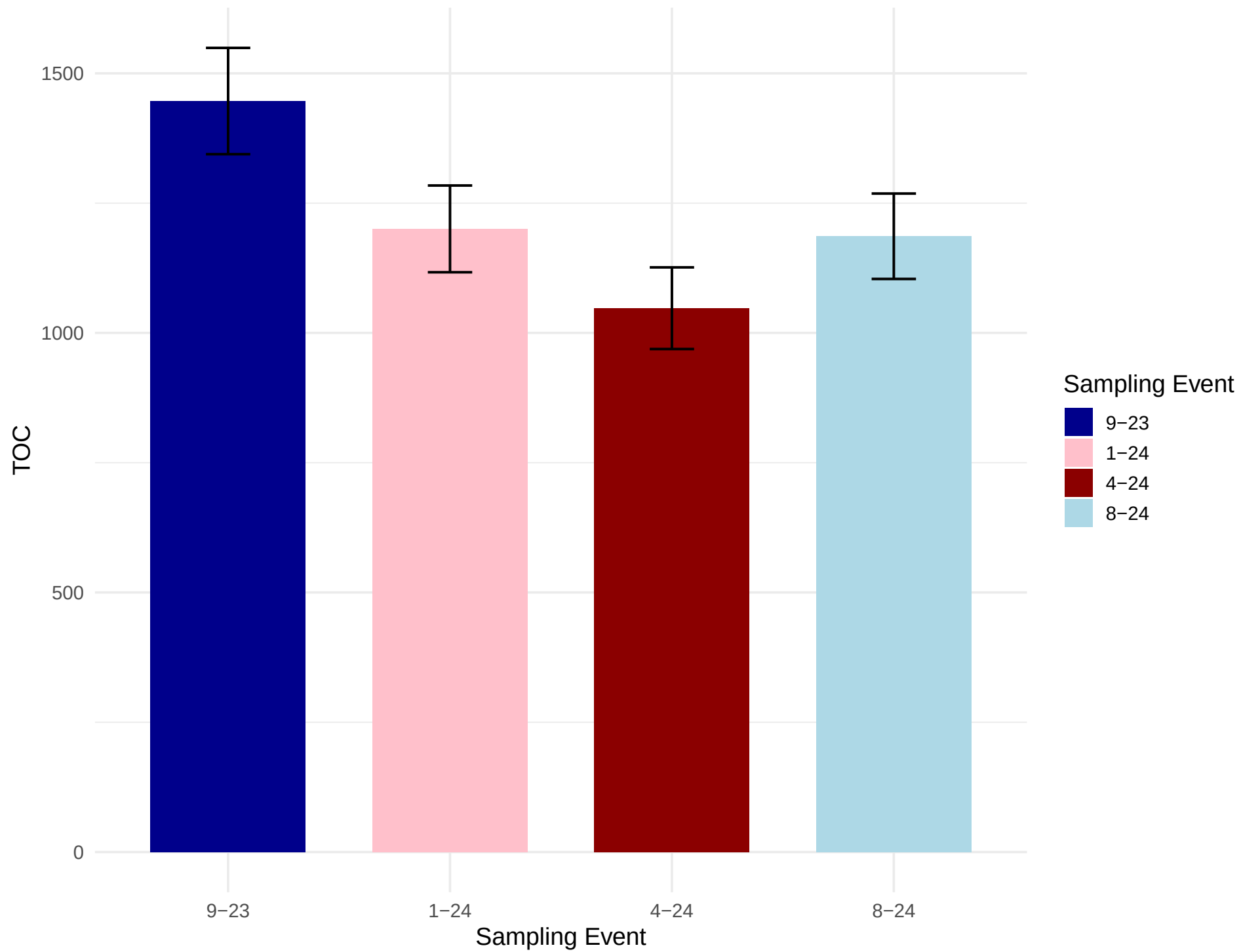
Average TOC across Sampling Events
