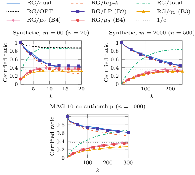
Figure 7: Hypergraph cut: certified approximation ratio of random greedy (RG, mean over trials) with respect to each upper bound, as a function of the cardinality k . f(S) = weight of hyperedges split by S ; random hypergraphs and the MAG-10 co-authorship hypergraph. RG/OPT uses the exact optimum (brute force) where it was computable. Additional baselines: the LP over the dual’s base sets (B2), the pruned double-greedy bound \gamma_1 (B3) and the modular bounds \mu_2 , \mu_3 on the pruned lattice (B4); B3 and B4 bound the unconstrained optimum. Curves are means over graph/sample seeds.
