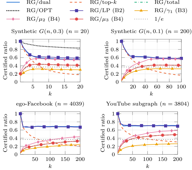
Figure 3: Revenue maximization: certified approximation ratio of random greedy (RG, mean over trials) with respect to each upper bound, as a function of the cardinality k . f(S) = \sum_{i \notin S} \sqrt{\sum_{j \in S} w_{ij}} with w_{ij} \sim U(0, 1) . RG/OPT uses the exact optimum (brute force) where it was computable. On the largest instances the dual bound is minimized over every 5th or 10th greedy prefix only. Additional baselines: the LP over the dual’s base sets (B2), the pruned double-greedy bound \gamma_1 (B3) and the modular bounds \mu_2, \mu_3 on the pruned lattice (B4); B3 and B4 bound the unconstrained optimum. Curves are means over graph/sample seeds.
