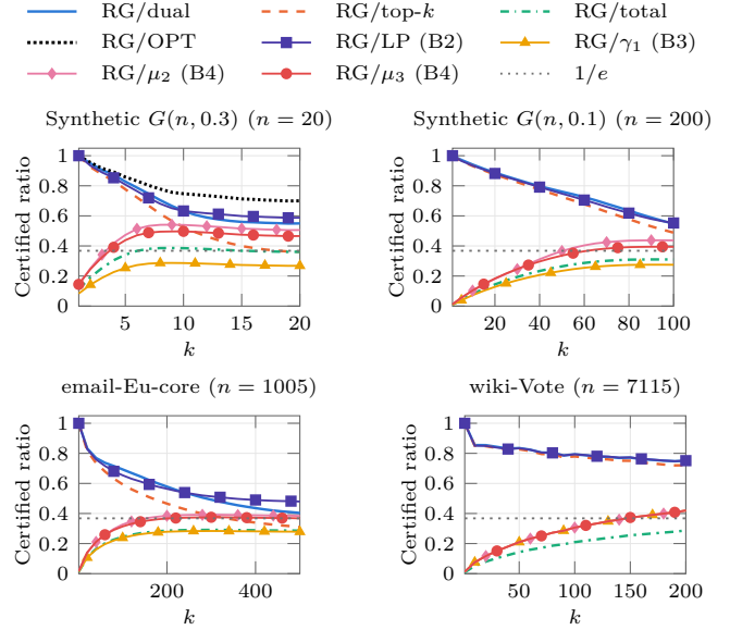
Figure 2: Directed cut: certified approximation ratio of random greedy (RG, mean over trials) with respect to each upper bound, as a function of the cardinality k . f(S) = weight of edges leaving S ; synthetic G(n, p) with random orientations and SNAP graphs. RG/OPT uses the exact optimum (brute force) where it was computable. On the largest instances the dual bound is minimized over every 10th greedy prefix only. Additional baselines: the LP over the dual's base sets (B2), the pruned double-greedy bound \gamma_1 (B3) and the modular bounds \mu_2, \mu_3 on the pruned lattice (B4); B3 and B4 bound the unconstrained optimum. Curves are means over graph/sample seeds.
