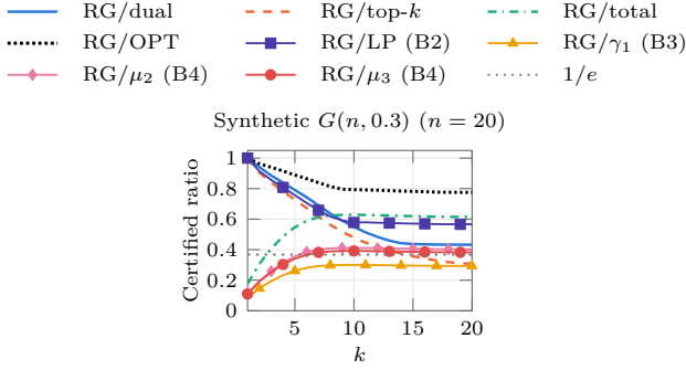
Figure 1: Max-cut: certified approximation ratio of random greedy (RG, mean over trials) with respect to each upper bound, as a function of the cardinality k . f(S) = weight of edges crossing (S, V \setminus S) ; G(n, p) with integer weights in \{1, \dots, 9\} . RG/OPT uses the exact optimum (brute force) where it was computable. Additional baselines: the LP over the dual's base sets (B2), the pruned double-greedy bound \gamma_1 (B3) and the modular bounds \mu_2, \mu_3 on the pruned lattice (B4); B3 and B4 bound the unconstrained optimum. Curves are means over graph/sample seeds.
