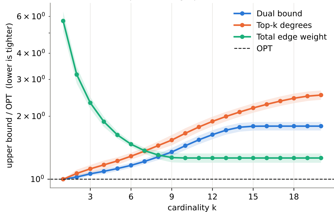
Upper bounds relative to OPT G(n=20, p=0.3) , 10 graph seeds, mean \pm 1 sd
