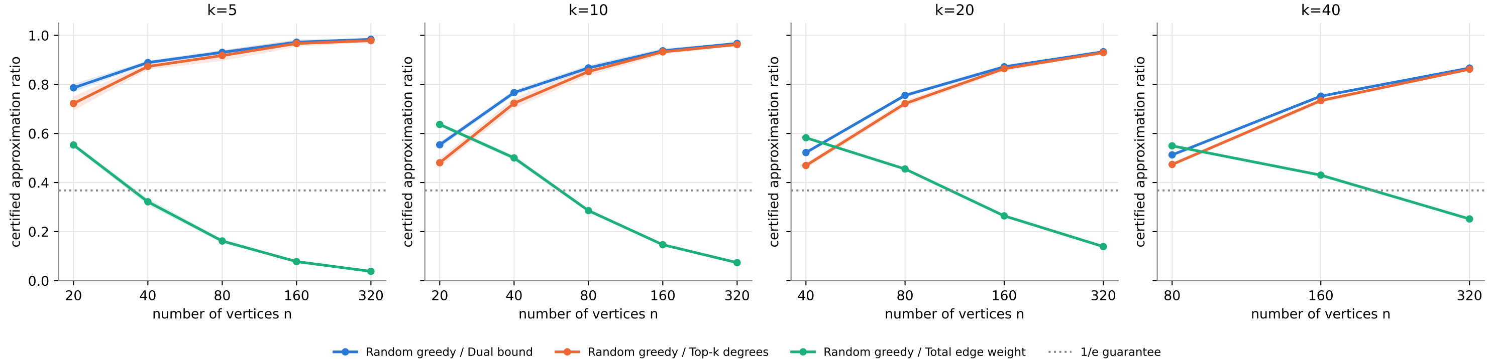
Certified ratio of Random greedy as n grows ( p=0.3 ; OPT unknown for n>20 )
