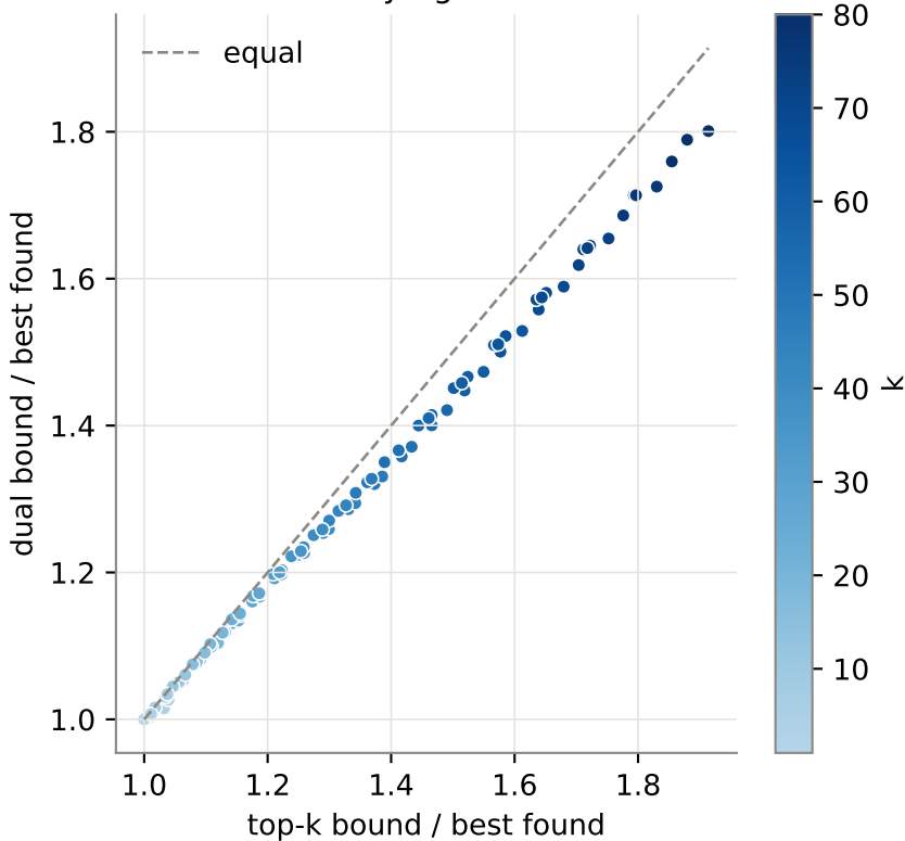
Per-run comparison (105 runs) dual strictly tighter in 95%
