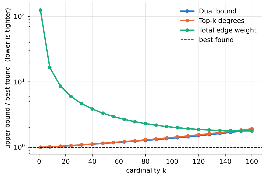
Upper bounds relative to best found G(n=320, p=0.3) , 5 graph seeds, mean \pm 1 sd
