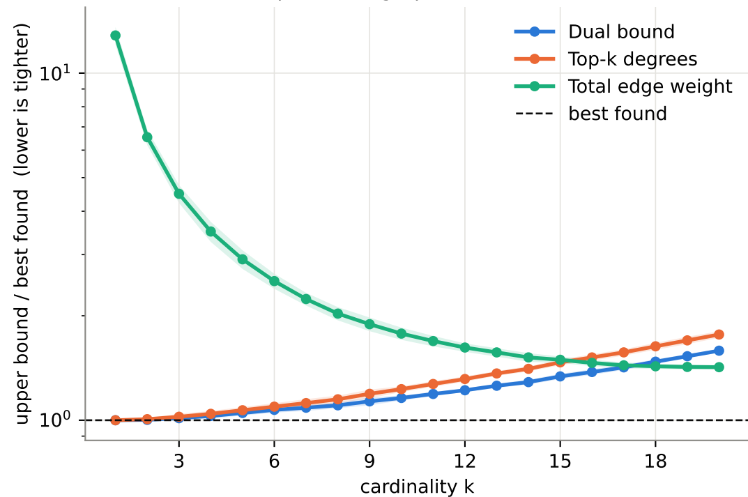
Upper bounds relative to best found G(n=40, p=0.3) , 5 graph seeds, mean \pm 1 sd
