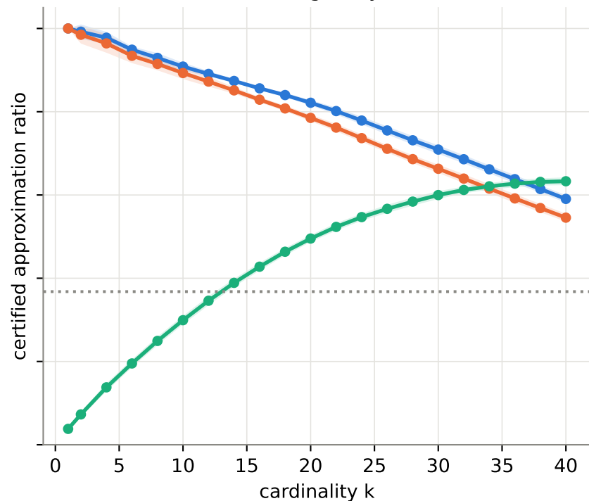
Plain greedy
