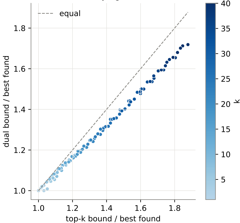
Per-run comparison (105 runs) dual strictly tighter in 91%
