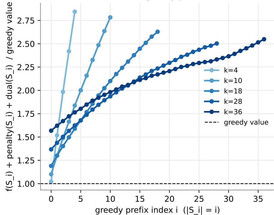
Bound obtained from each greedy prefix (mean over seeds)
