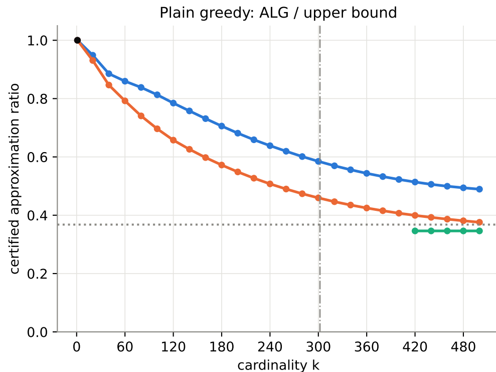
Directed cut — email-Eu-core (n=1005, 1 seed, mean \pm 1 sd)
