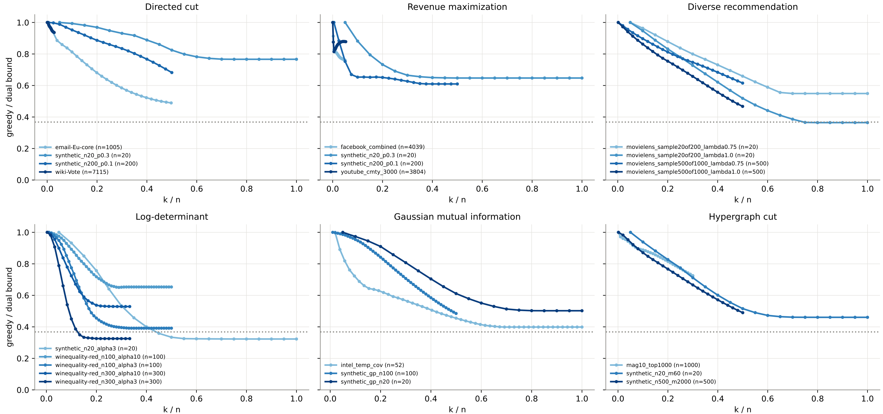
Certified ratio of plain greedy from the dual bound (dotted: 1/e )
