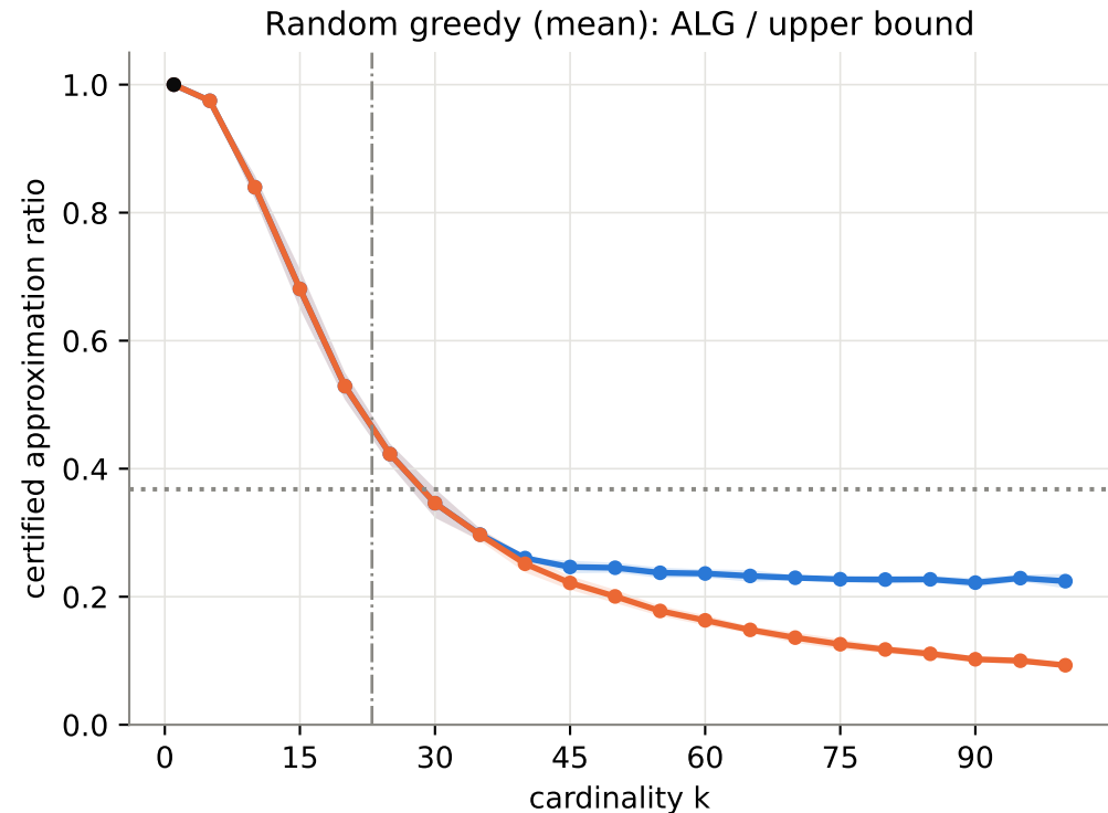
Log-determinant — winequality-red_n300_alpha3 (n=300, 2 seeds, mean \pm 1 sd, dual over every 5th greedy prefix)
