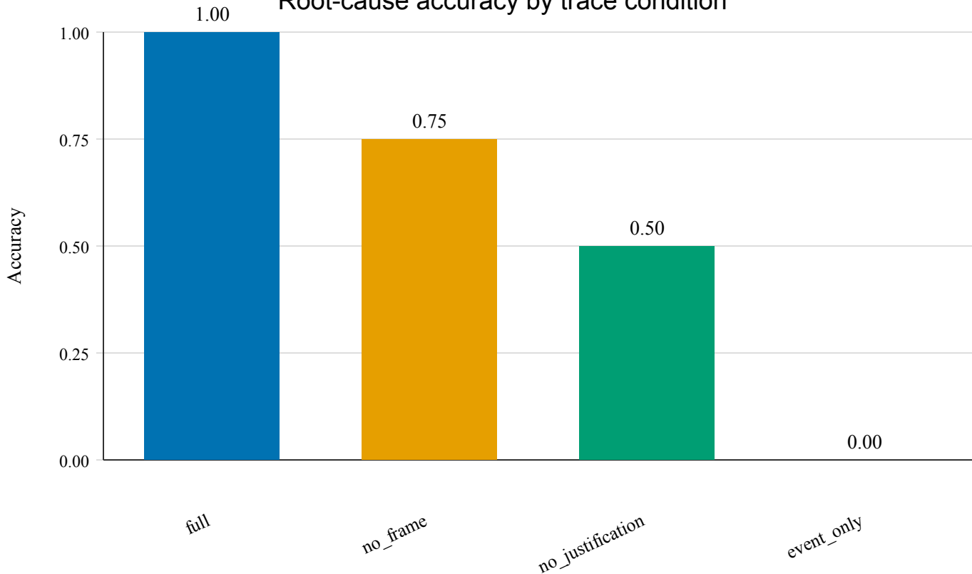
Root-cause accuracy by trace condition
