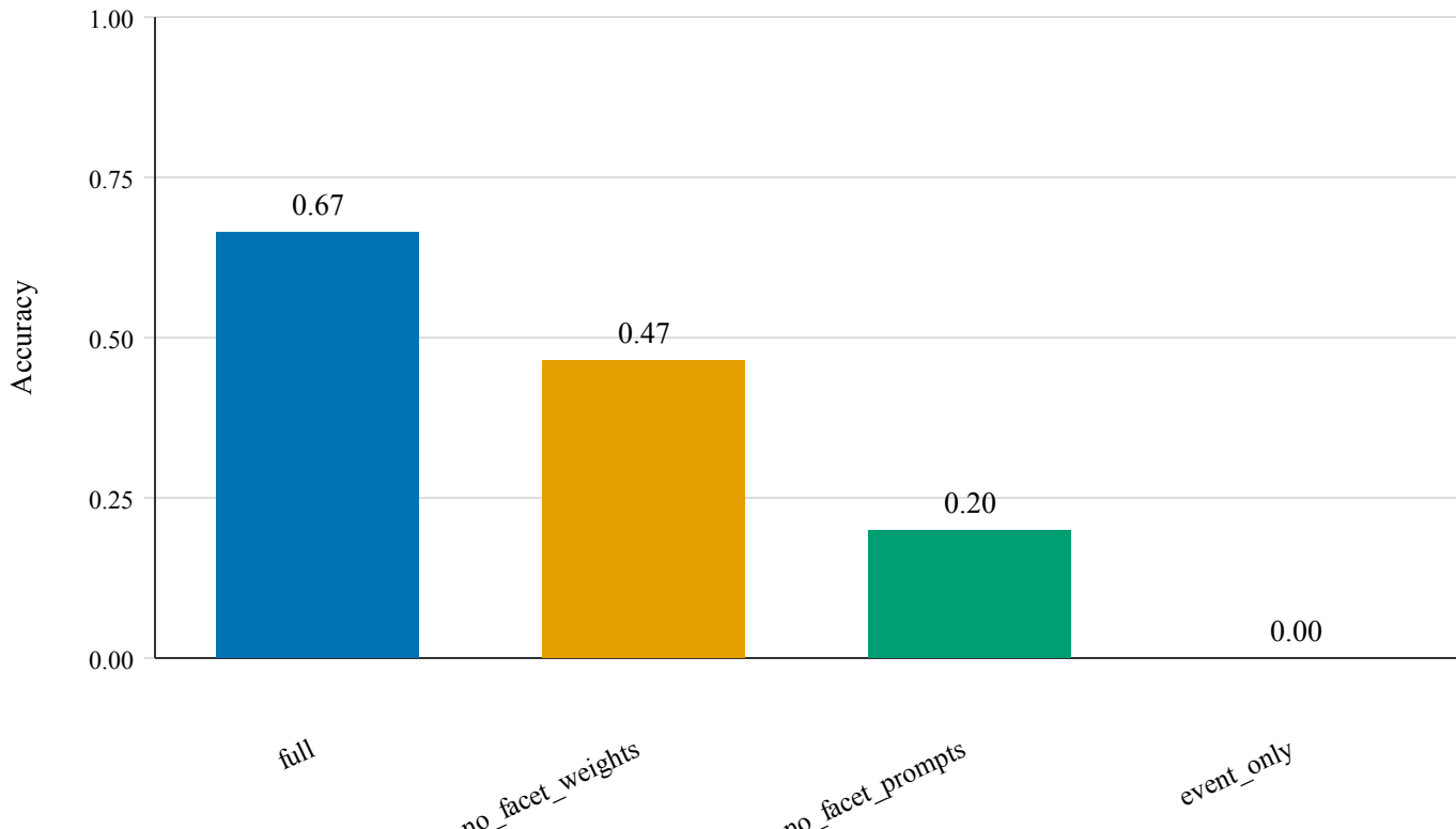
Persona faithfulness accuracy by trace condition
