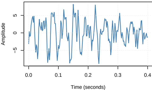
Input EEG Signal x3
