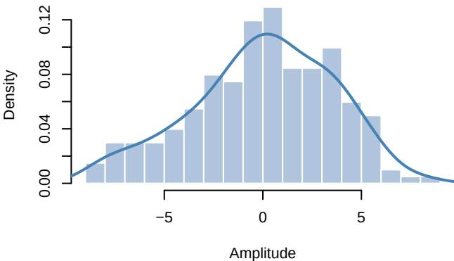
Distribution of Input Signal x3
