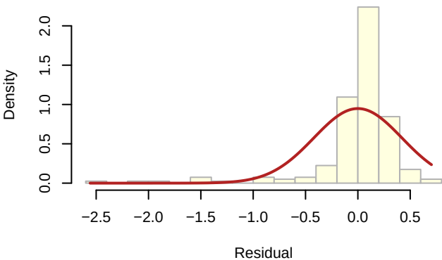
Residual Distribution – Model 3
