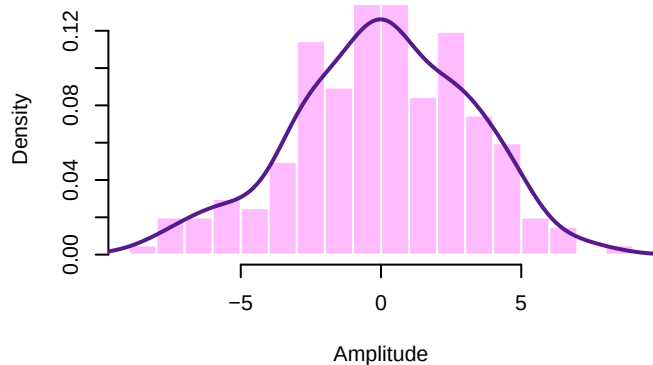
Distribution of Input Signal x4
