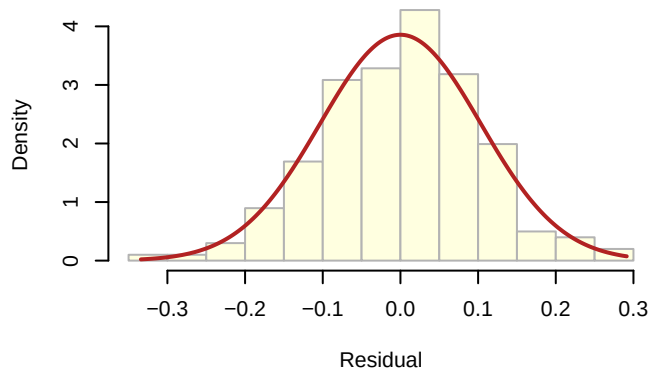
Residual Distribution – Model 4
