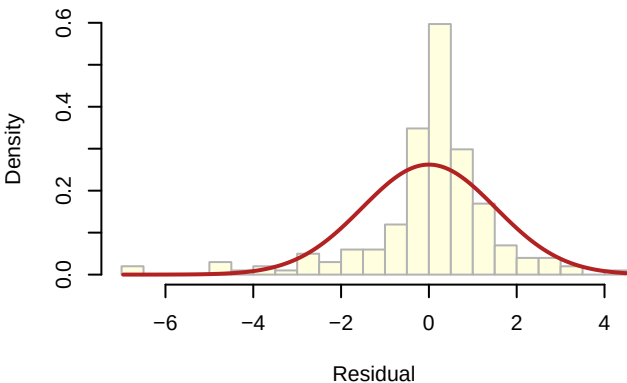
Residual Distribution – Model 5
