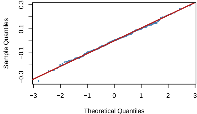
Q-Q Plot – Model 4
