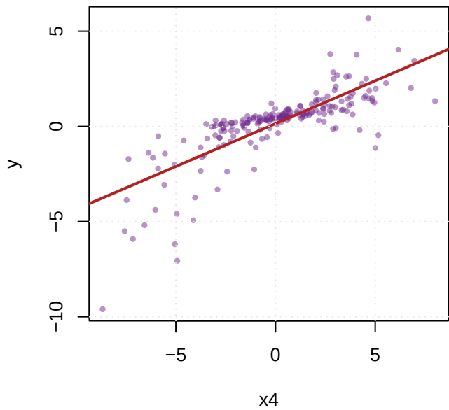
x4 vs y ( r = 0.7747 )
