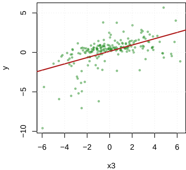
x3 vs y ( r = 0.5255 )
