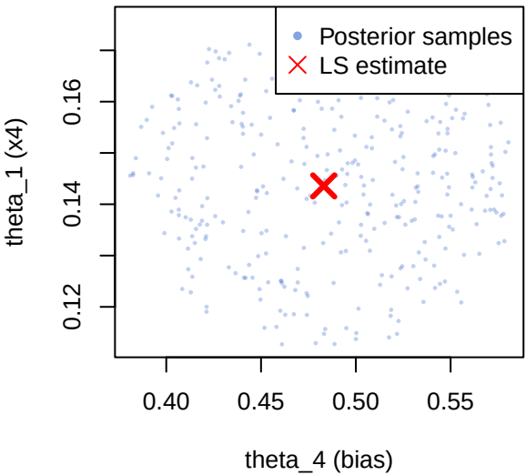
Joint Posterior Distribution (Rejection AE)
