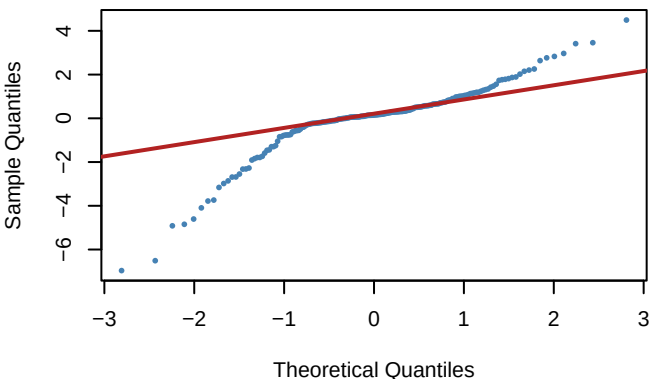
Q-Q Plot – Model 5
