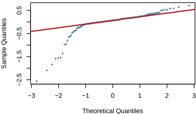
Q-Q Plot – Model 3
