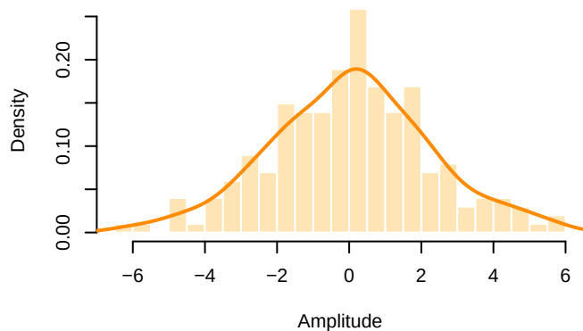
Distribution of Input Signal x4
