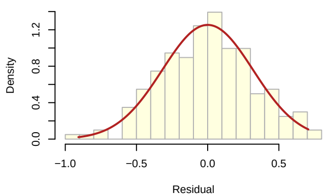
Residual Distribution – Model 4
