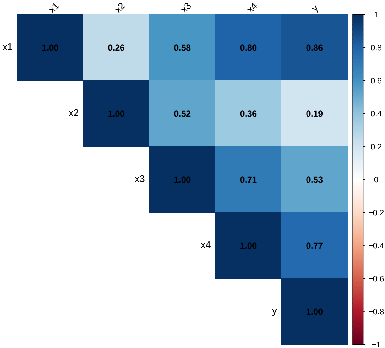
Correlation Heatmap of EEG Signals
