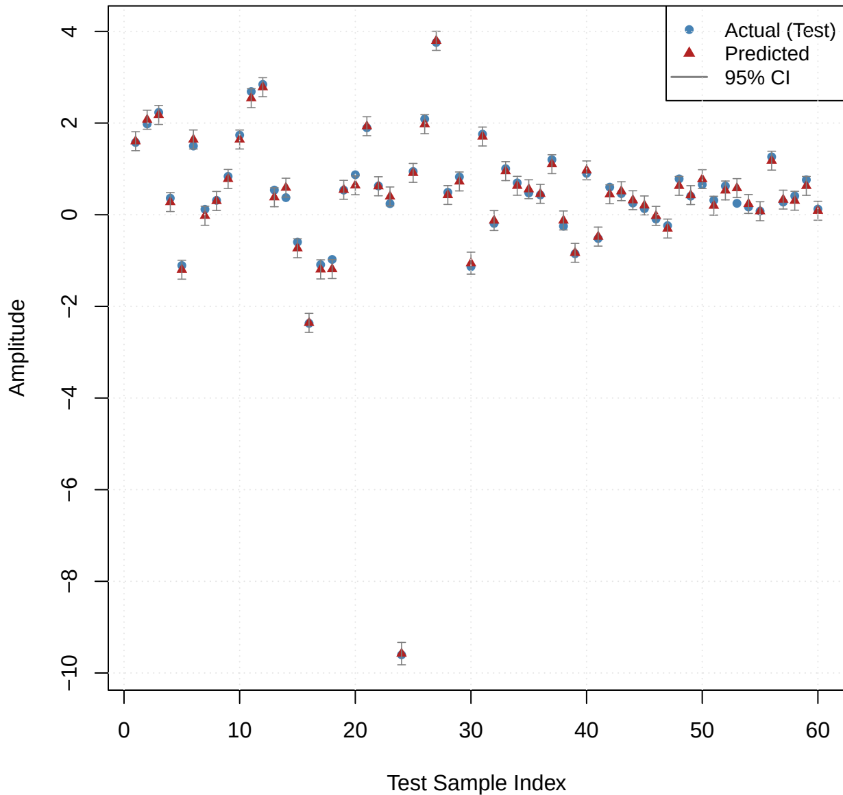
Model Prediction with 95% CI – Model 2
