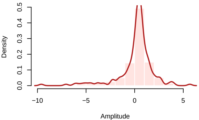
Distribution of Output Signal y
