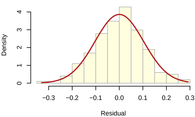
Residual Distribution – Model 5
