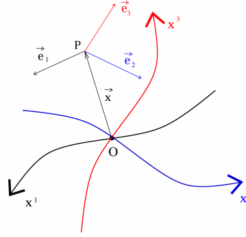
Figura 4.9: Vector tangentes.
