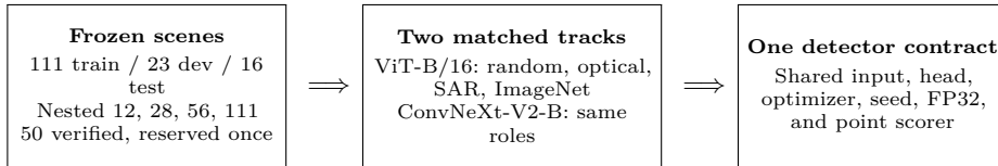
Fig. 1. Controlled study design. Initialization is the only variable within each architecture track. Matched roles are compared descriptively across tracks; the final human-verified set remains sealed until the cohort and analysis code are frozen.
