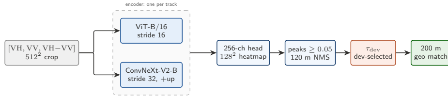
Fig. 3. The shared detection path: only the encoder differs by track; one head, decode rule, dev-selected threshold, and frozen scorer serve every arm.
