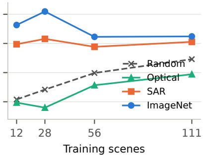
ConvNeXt-V2-Base
