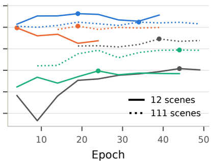
ConvNeXt-V2-Base
