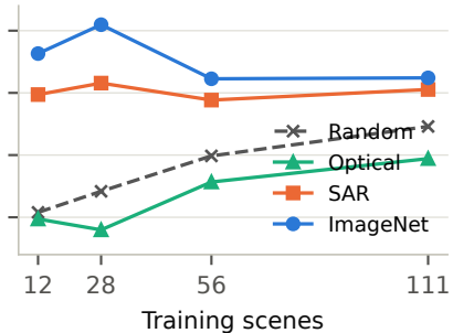
ConvNeXt-V2-Base
