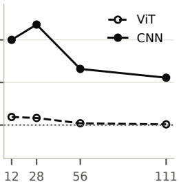
SAR – optical
