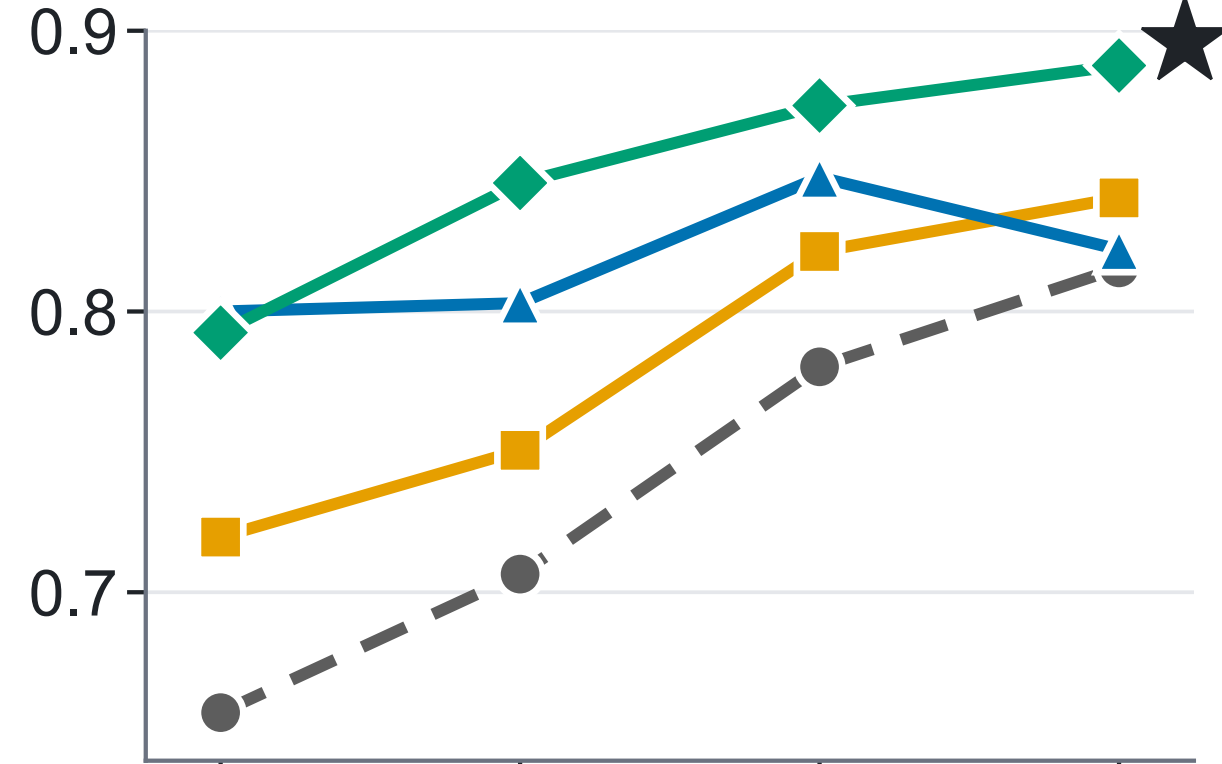
ConvNeXt-V2-Base
