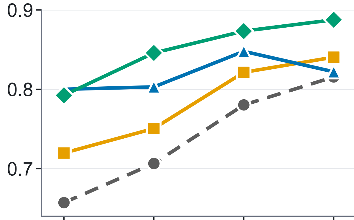
ConvNeXt-V2-Base
