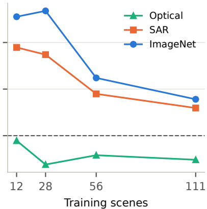
ConvNeXt-V2-Base
