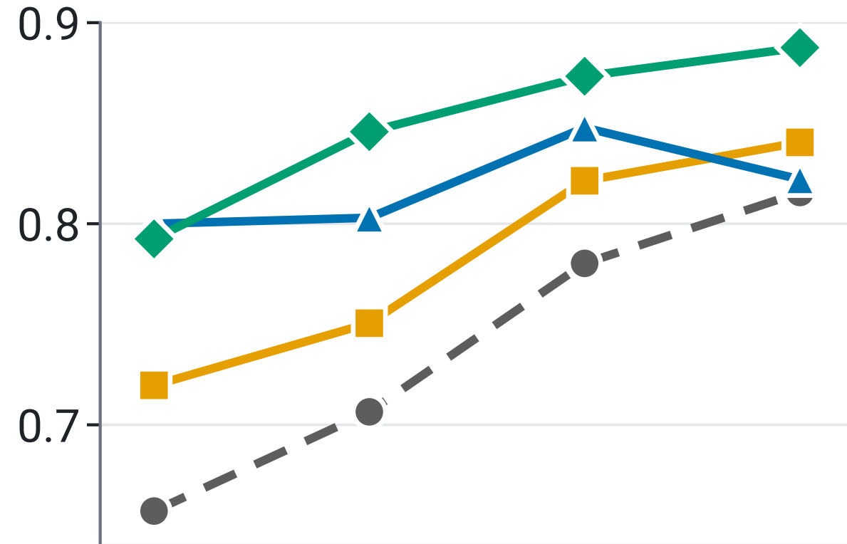
ConvNeXt-V2-Base
