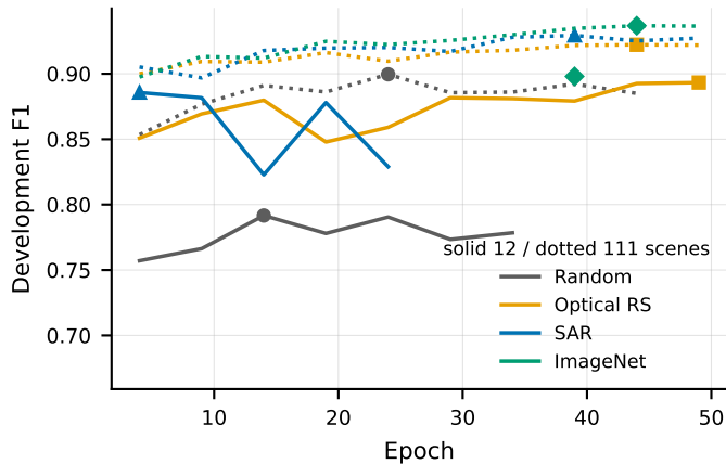
ViT-B/16 track
