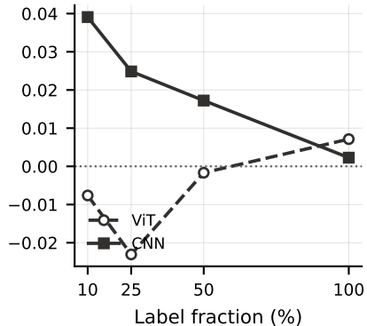
SAR – optical
