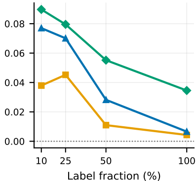
ConvNeXt-V2-B track
