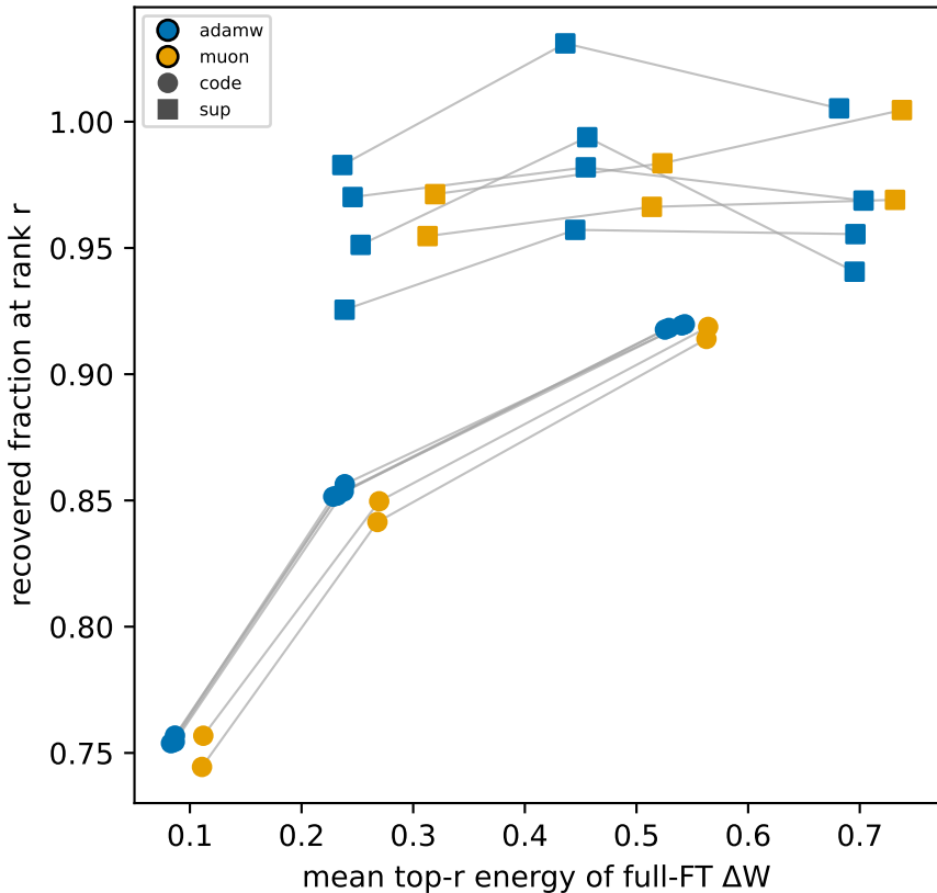
does \Delta W spectrum predict the LoRA gap? ( \rho = 0.62 )
