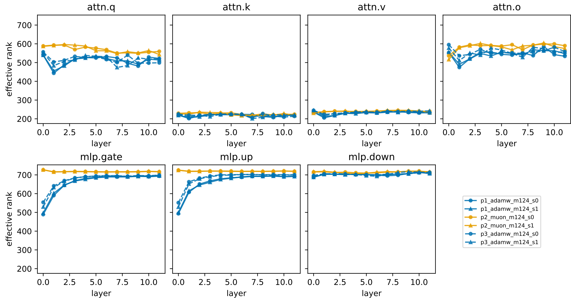
H1: effective rank of pretrained weights by layer
