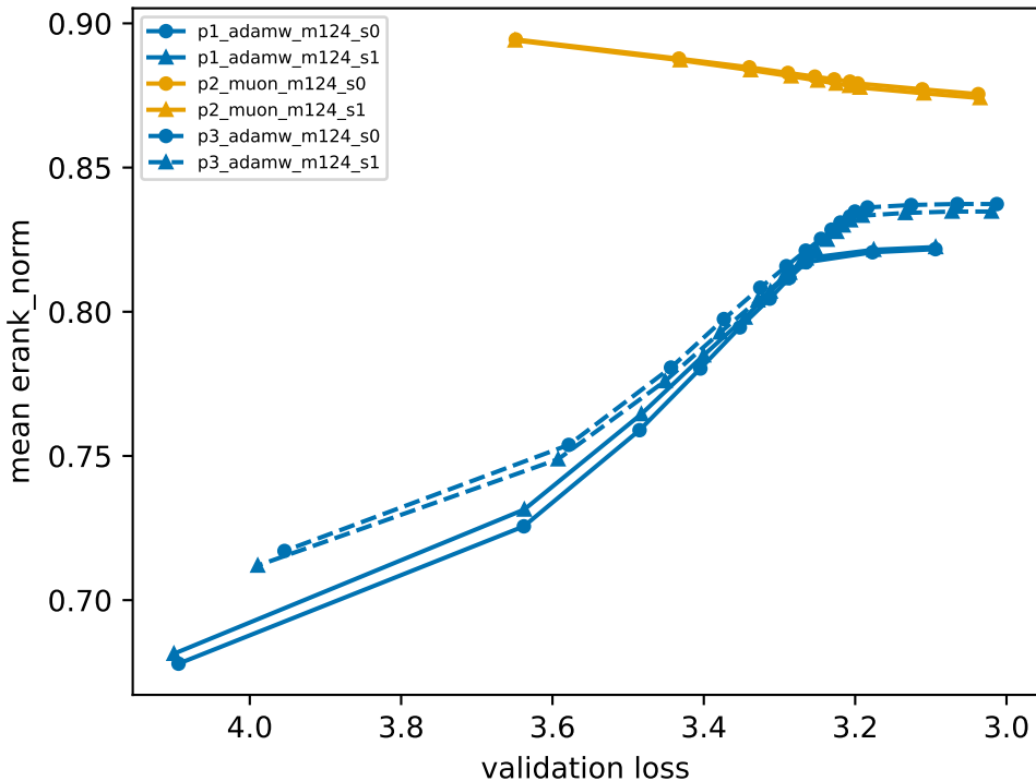
H1: effective rank versus training progress
