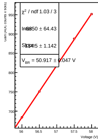
Gain vs Voltage for ADC 0, Channel 5
