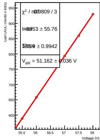
Gain vs Voltage for ADC 0, Channel 4
