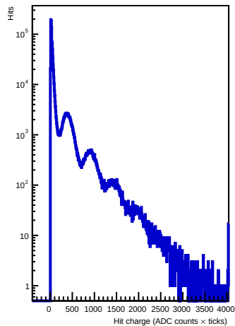
Run 1133 - adc 0 - ch 4 - 57.0V
