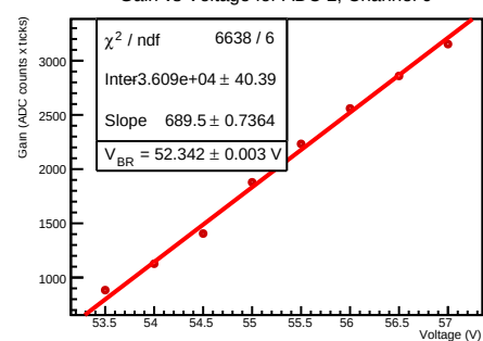
Gain vs Voltage for ADC 2, Channel 6
