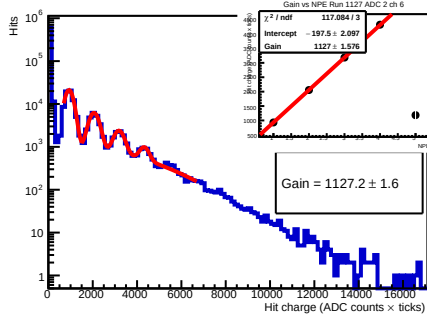
Run 1127 - adc 2 - ch 6 - 54.0V
