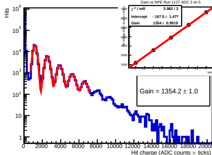
Run 1127 - adc 2 - ch 5 - 54.0V
