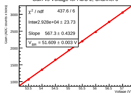
Gain vs Voltage for ADC 2, Channel 5
