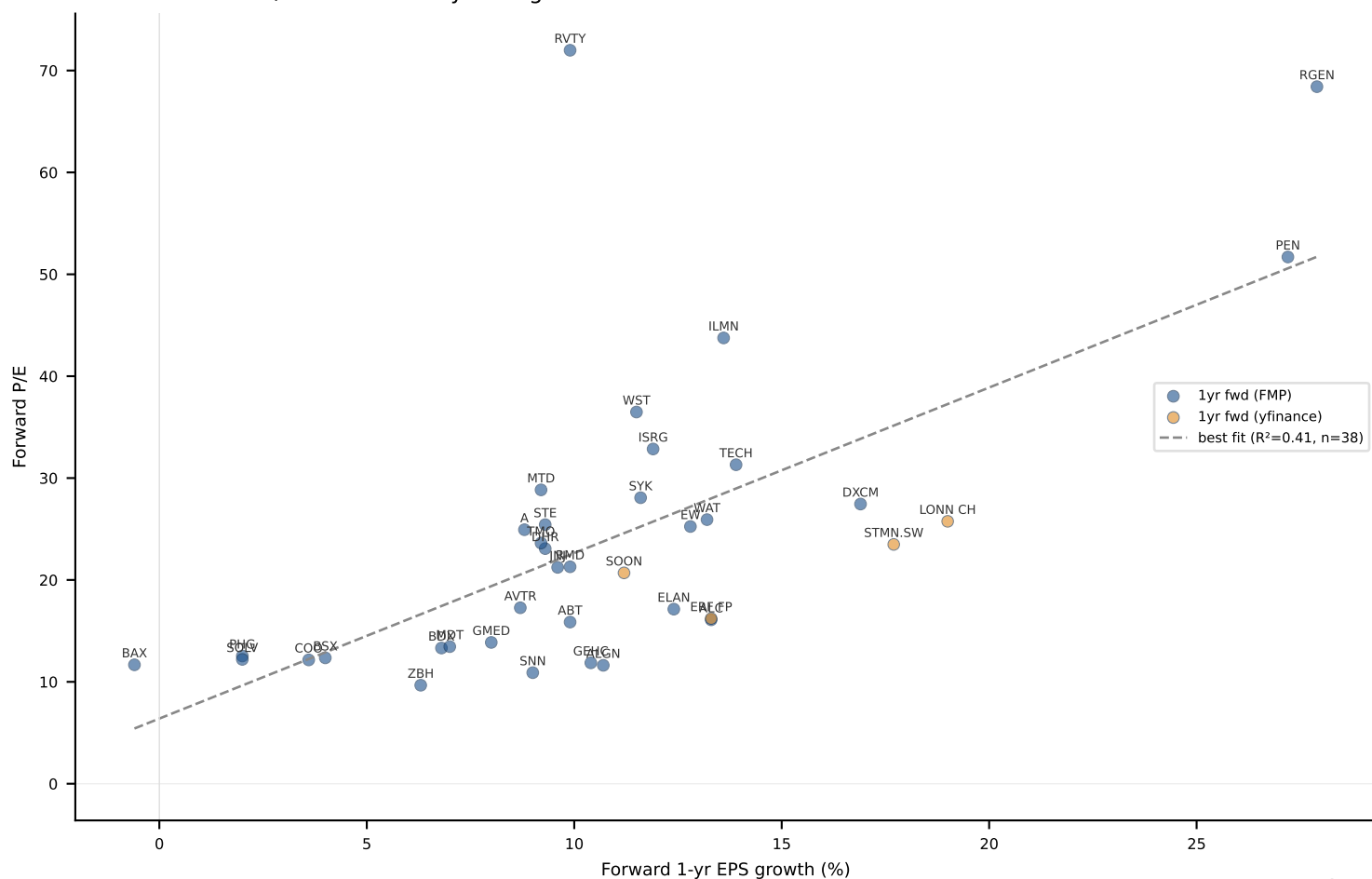
MedTech — Fwd P/E vs forward 1-yr EPS growth — 38 stocks
