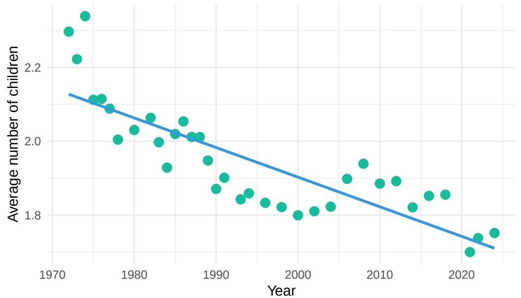
Scatterplot of Average Number of Children
