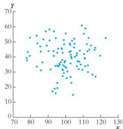
(c) Correlation = 0.0
