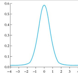
(b) Skewness = 0, kurtosis = 20
