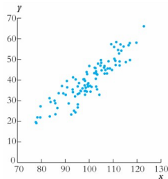
(a) Correlation = +0.9
