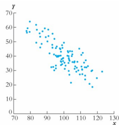
(b) Correlation = -0.8
